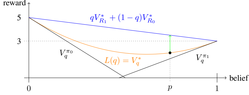
Figure 1: The agent is uncertain between two reward functions R_0 and R_1 . The horizontal axis shows the current belief p over R_1 ; q = 0 corresponds to certainty in R_0 and q = 1 corresponds to certainty in R_1 . According to Proposition 2, the graph of the function L (orange parabola) is convex and bounded from above by the convex combination of the to the extreme values V_{R_0}^* = 5 and V_{R_1}^* = 3 (blue line). Moreover, it is bounded from below by the values of the two policies maximizing R_0 and R_1 . If our current belief is p , then the current optimal value V_p^* is found at the black dot. We want to incentivize the agent to perform actions that increase the information about the reward function without increasing bias, i.e., moving along the green arrow. We want to disincentivize the agent to perform actions that manipulate the information about the reward function, i.e., moving orthogonal to the green arrow (in expectation).
